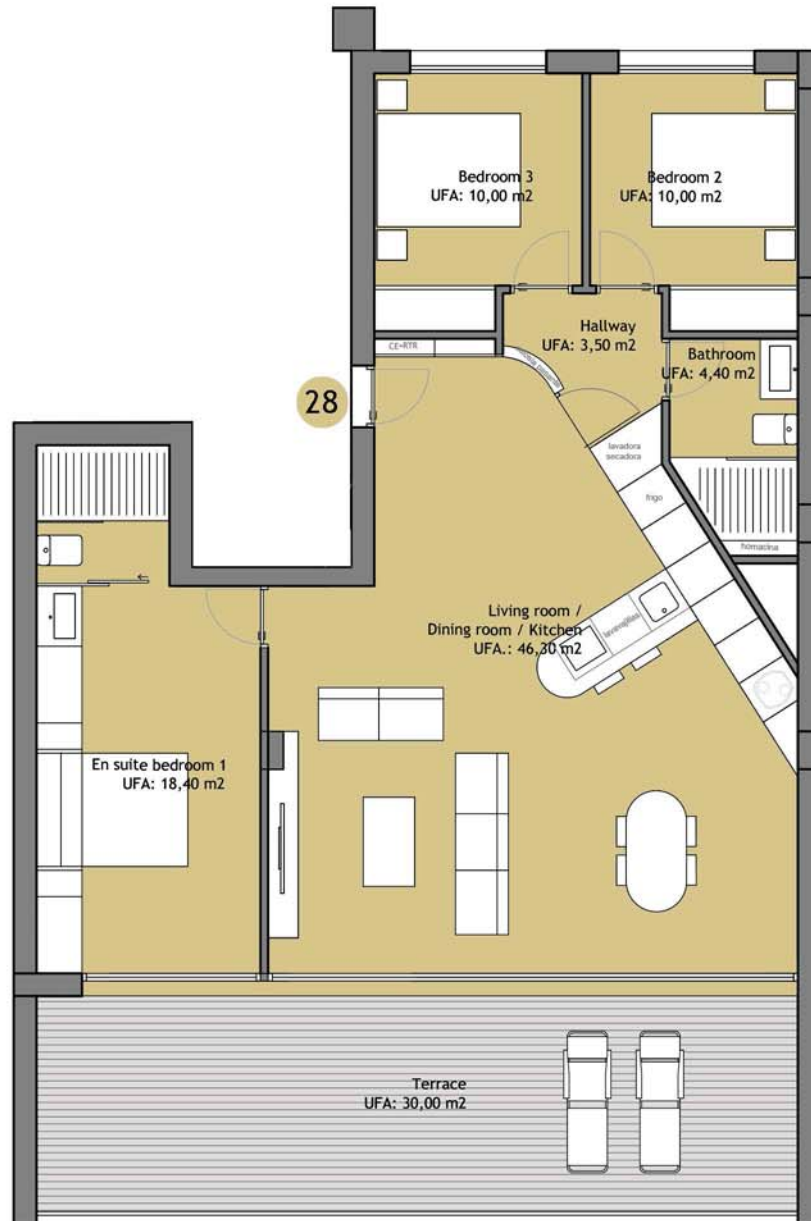
First Floor
