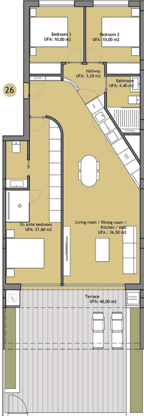
Ground Floor
